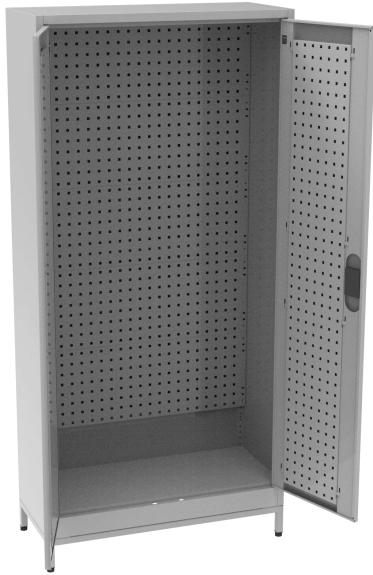
MPC-01 W900 D400 H1925 mm
